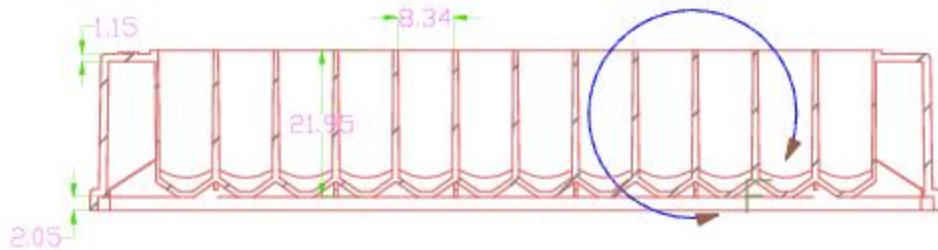
SECTION E-E
